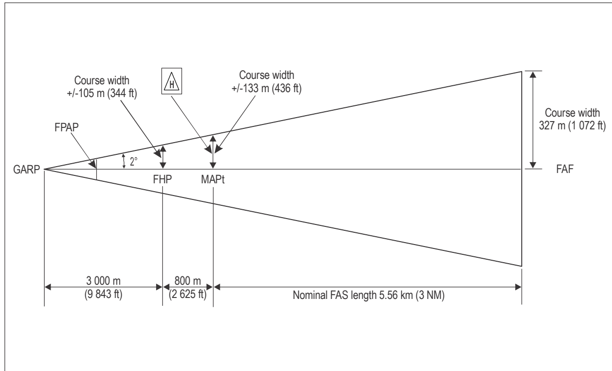
Figure IV-3-App B-1. Fictitious helipoint orientation and lateral display scaling
