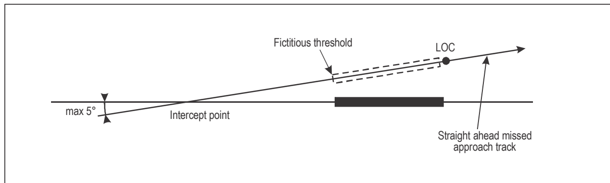
Figure II-1-2-1. Offset localizer
