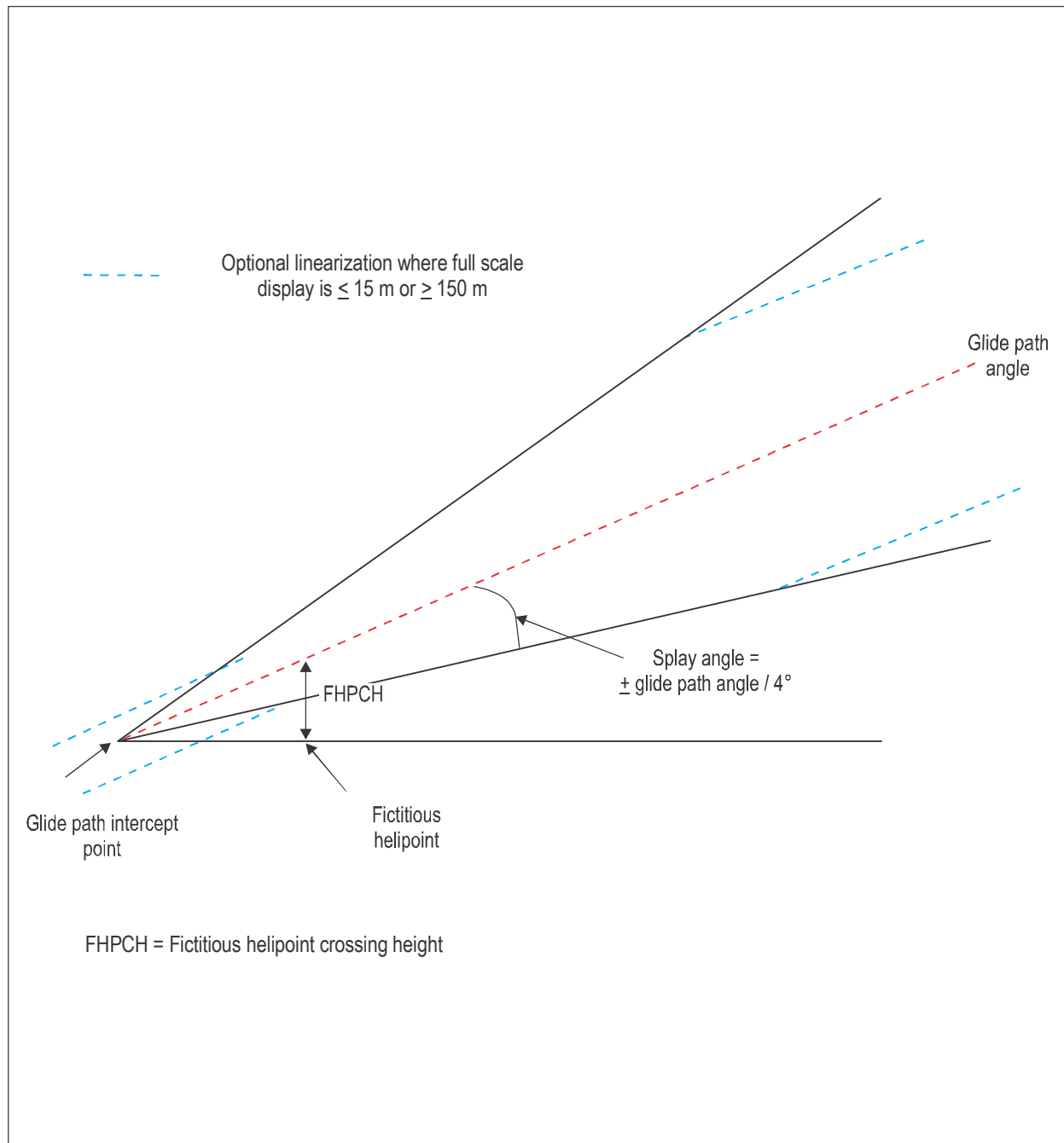
Figure IV-3-App B-2. Fictitious heliport orientation and vertical display scaling
