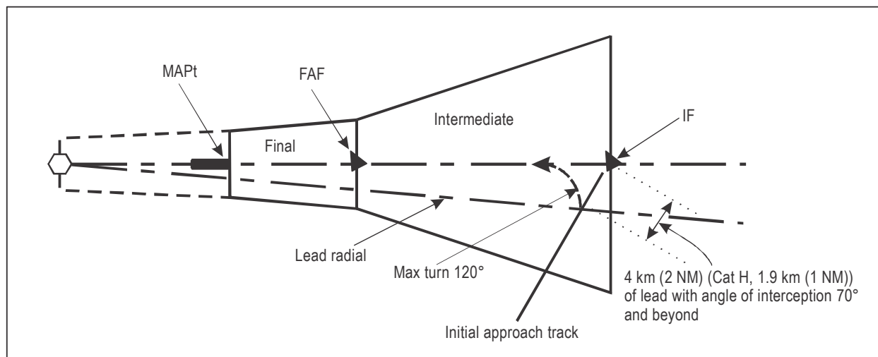
Figure I-4-3-1. Lead radial for turns greater than 70°
