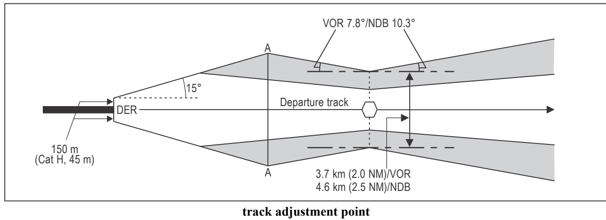
Figure I-3-3-4. Straight departure (facility ahead)
