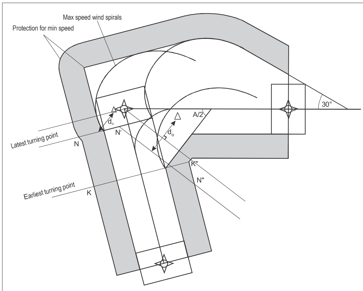
Figure III-3-2-3. Turn at a fly-by waypoint
