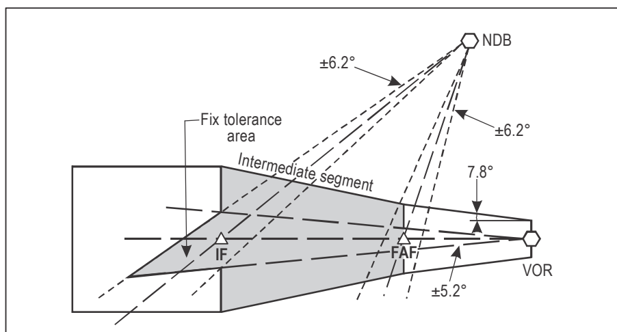
Figure I-2-2-9. Area requiring obstacle clearance
