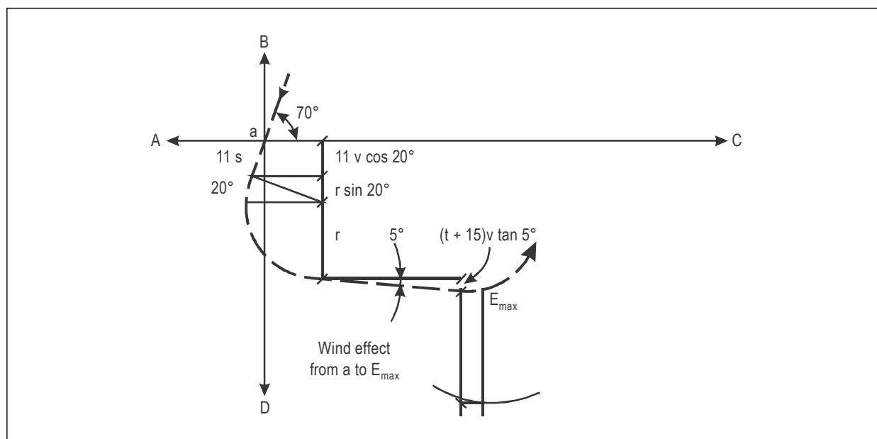
Figure I-4-3-App C-9.
