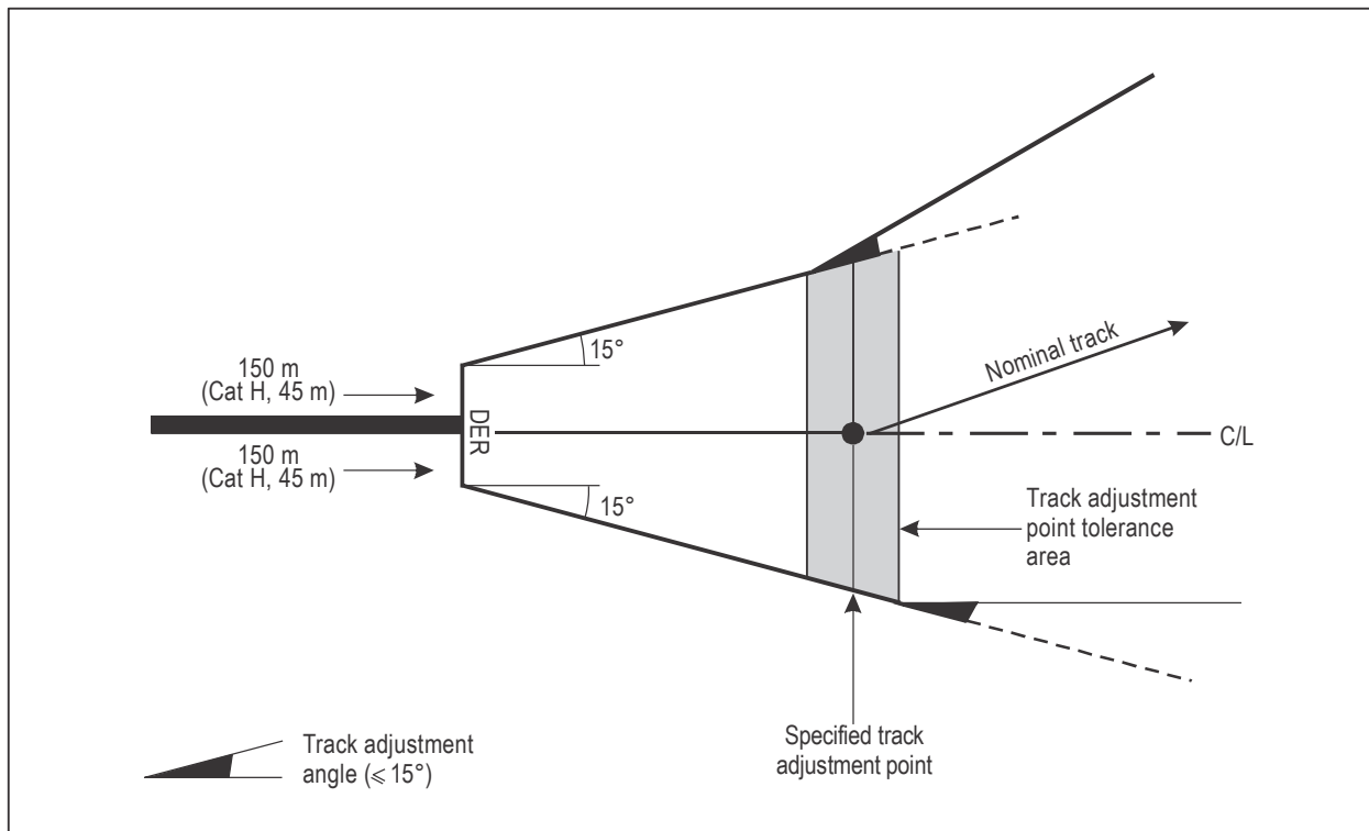
Figure I-3-3-3. Straight departure area with a specified
